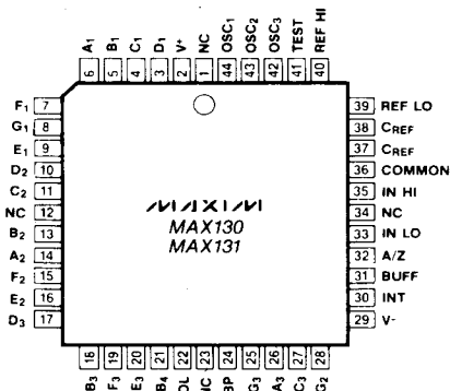
44 Lead Plastic Chip Carrier (Quad Pack)
