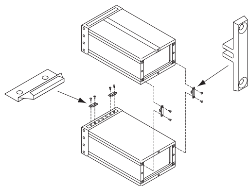
Vertical Connection
