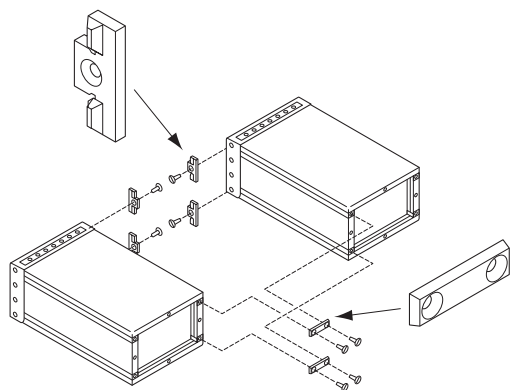
Side-by-side Connection
