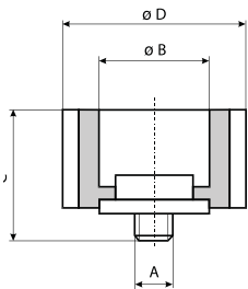
Gauge piece
