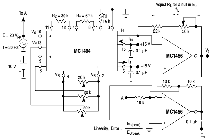
Figure 3. Linearity
