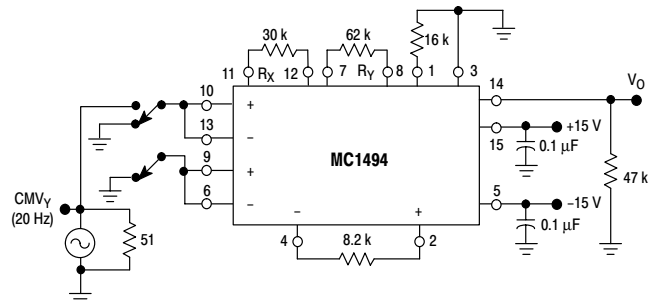
Figure 8. Common Mode
