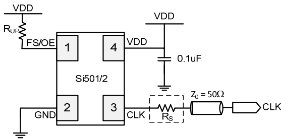
Si501/2 Apps Circuit w/ Optional Series Resistor
