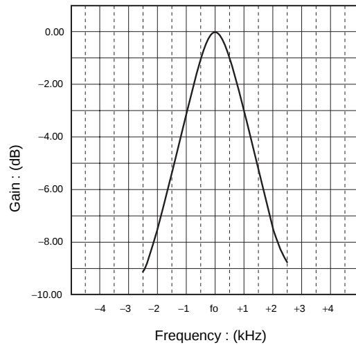
Fig.6 BPF characteristic
