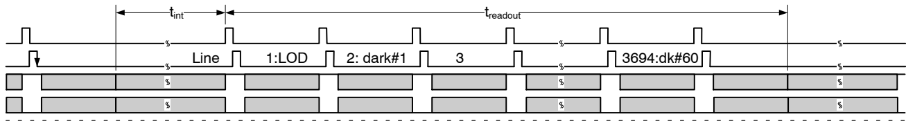
Figure 19. Frame Timing
