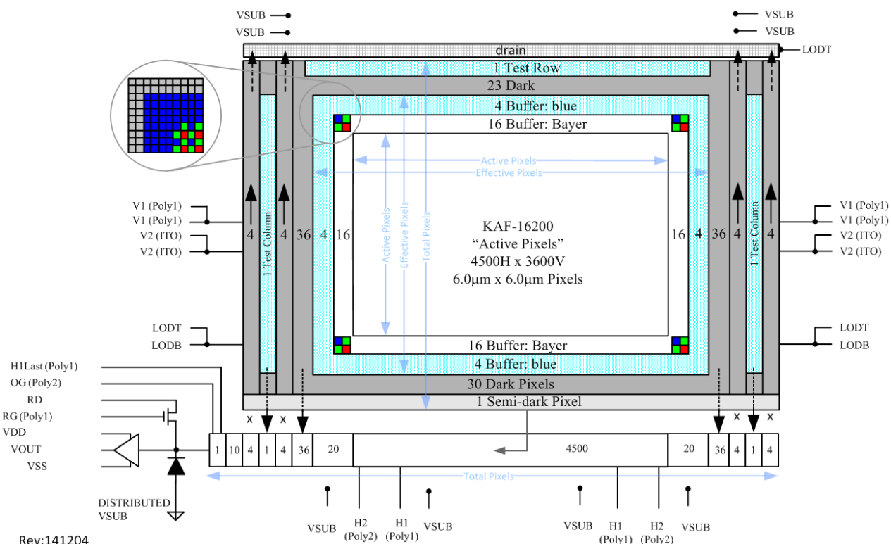
Figure 2. Block Diagram
