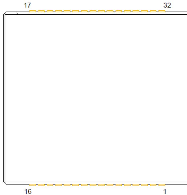
Figure 5. Pinout Diagram
