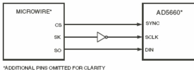
Figure 30. AD5660 to MICROWIRE Interface
