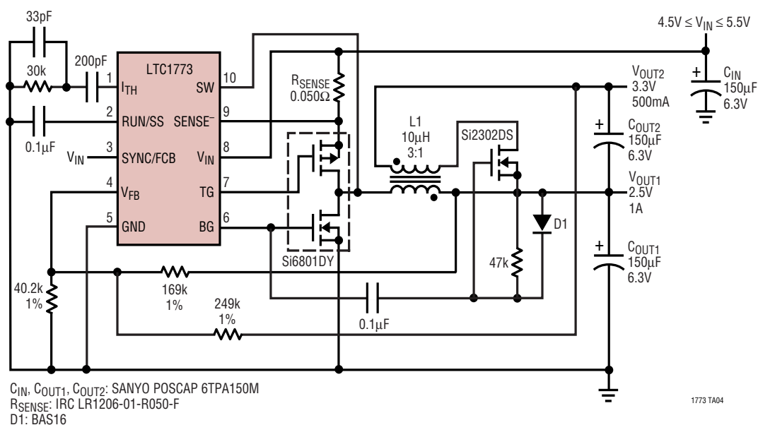
Figure 16. Dual Output Synchronous Buck Converter
