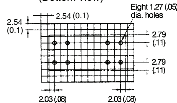
Dual coil (Bottom view)
