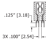
STAGGERED DIP SOLDER (HH)
