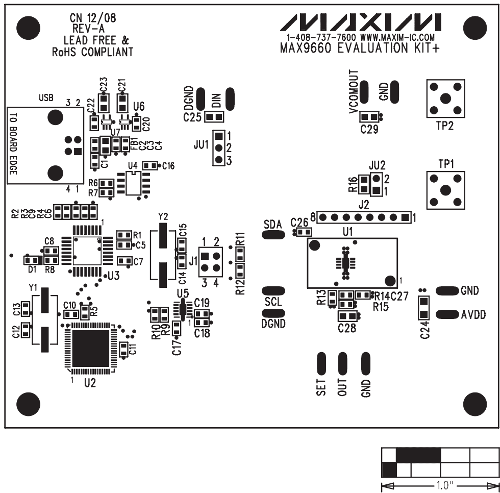
Figure 5. MAX9660 EV Kit Component Placement Guide—Component Side
