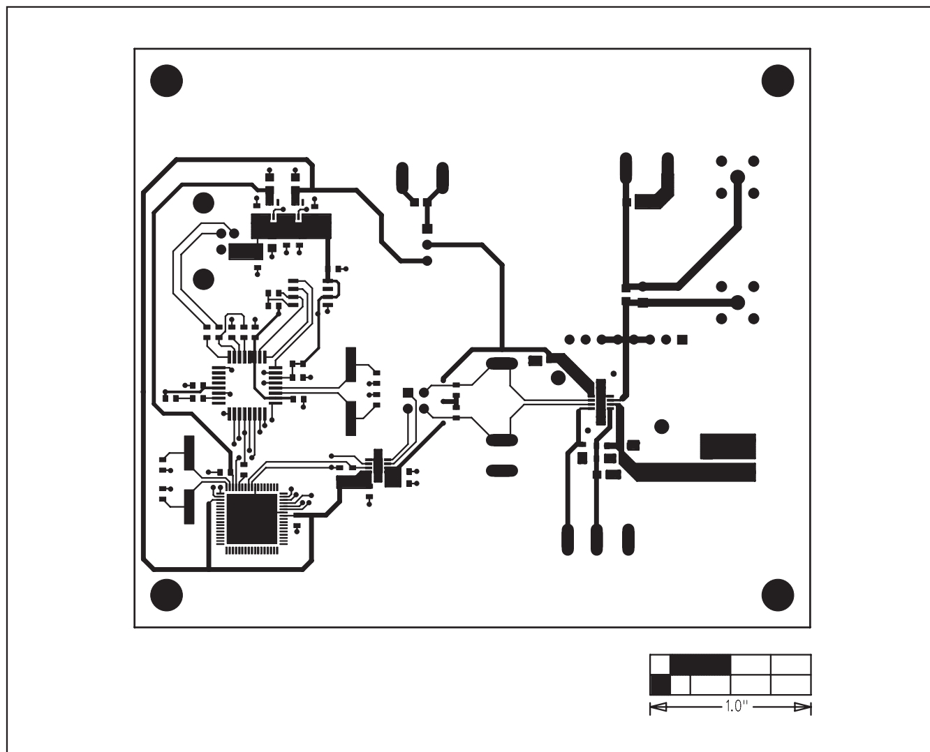
Figure 6. MAX9660 EV Kit PCB Layout—Component Side
