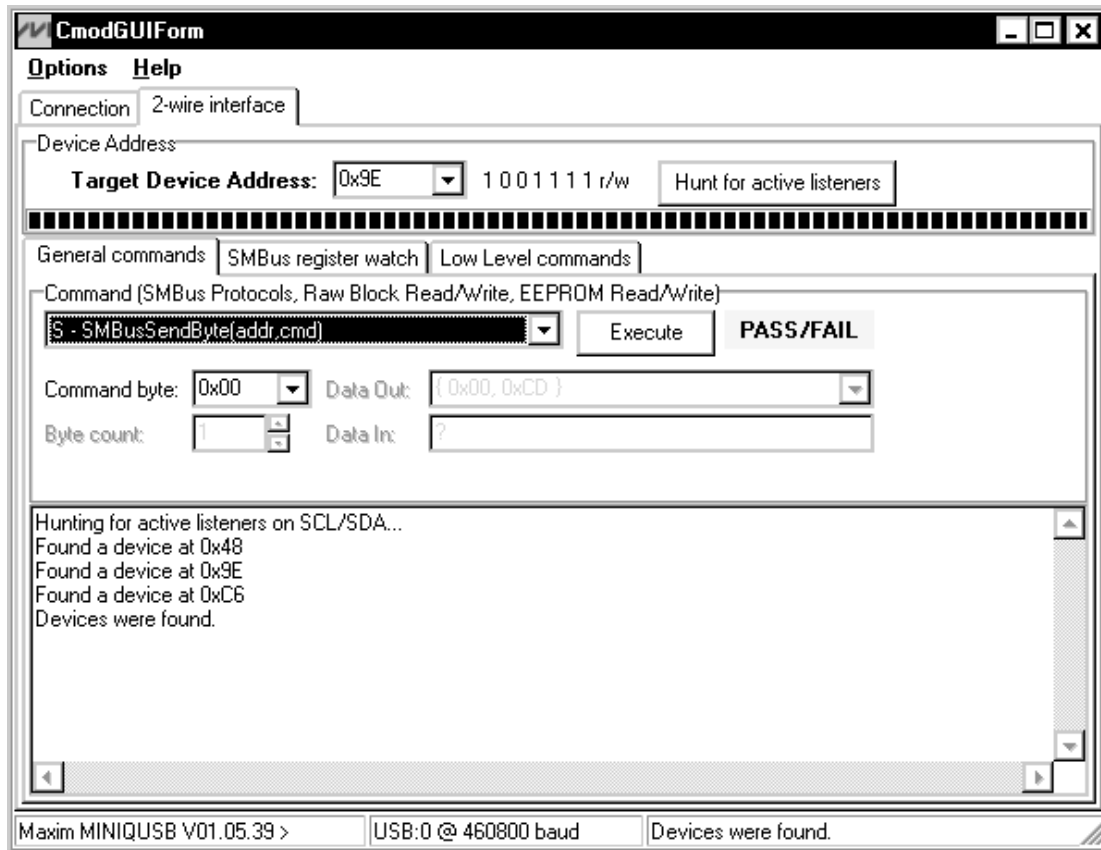
Figure 2. Advanced I 2 C User Interface Window (2-Wire Interface Tab)
