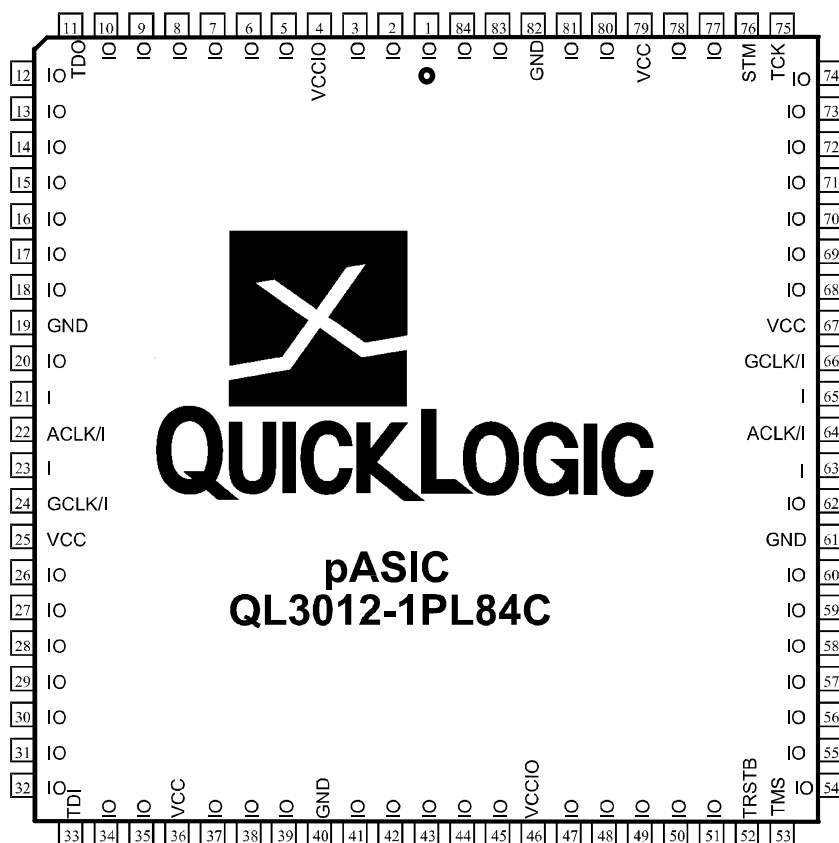
FIGURE 2. 84-Pin PLCC
