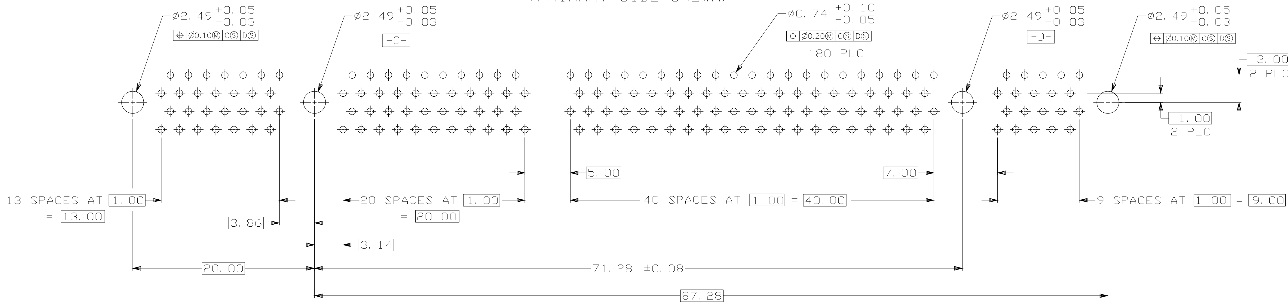
RECOMMENDED CONNECTOR MATING PAD PATTERN (PRIMARY SIDE SHOWN)
