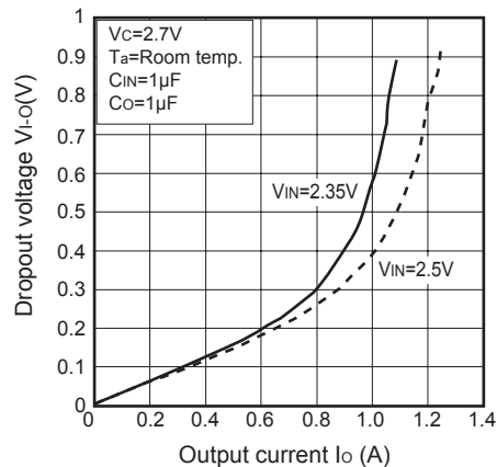
Fig.23 Dropout Voltage vs. Output Current (PQ025ENA1ZPH)
