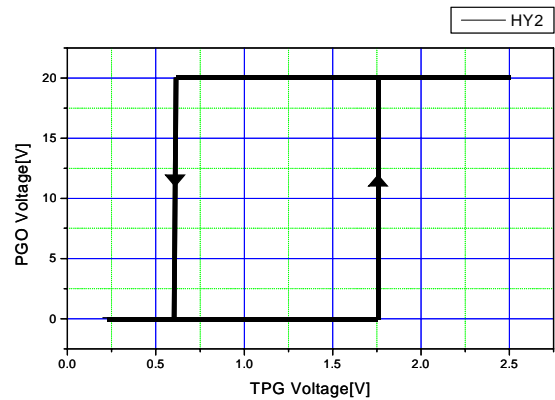
Figure 12. Hysteresis Voltage 2
