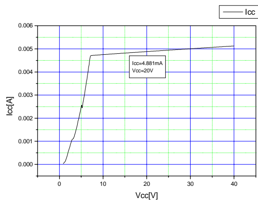
Figure 1. V_{CC} - I_{CC}
