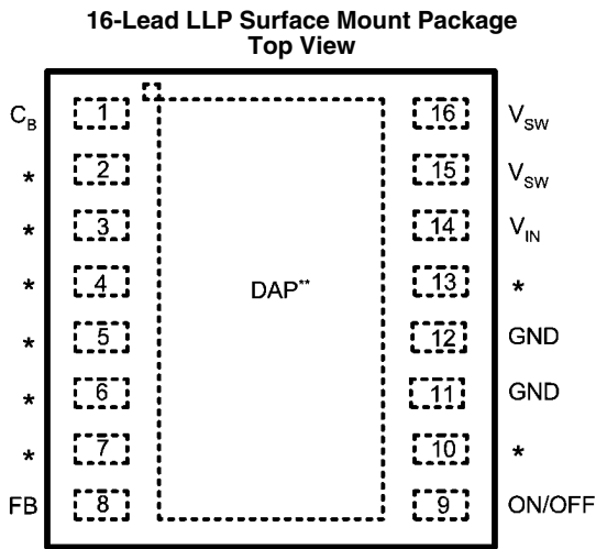
LLP Package See NSC Package Drawing Number LDA16A
