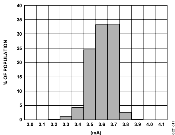
Figure 12. Current Consumption at 25°C ( V_{RATIO} = 5\text{ V} )
