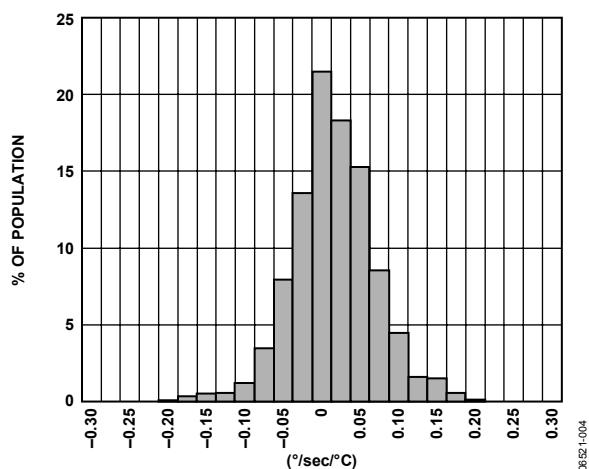
Figure 5. Null Drift over Temperature ( V_{RATIO} = 5\text{ V} )
