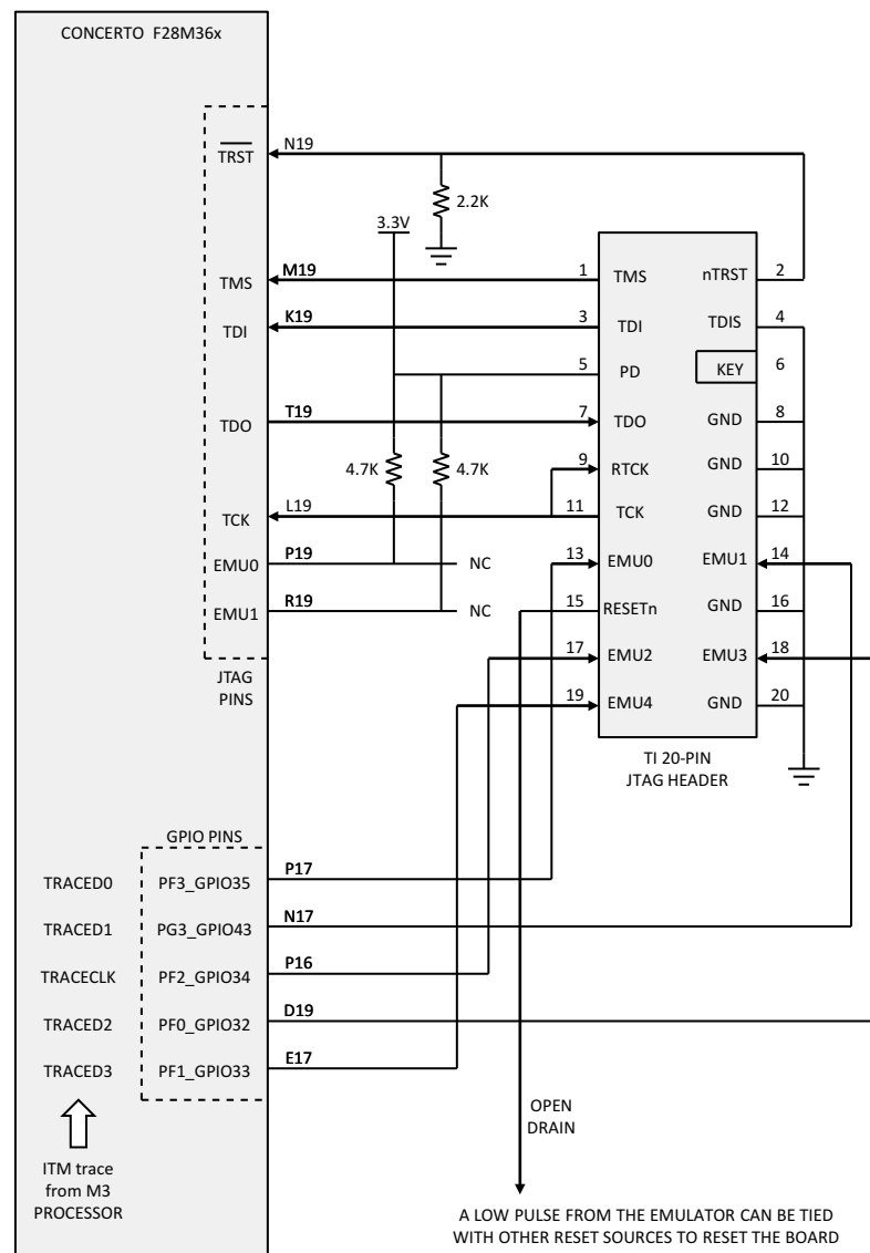
Figure 6-19. Connecting to TI 20-Pin JTAG Emulator Header
