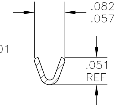
SECTION A-A SCALE 8:1
