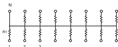
Schematic B Bussed
