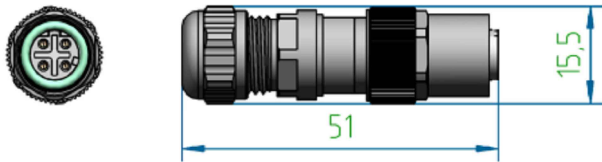
M12 D-4 FEMALE CABLE CLAMP RANGE FROM 4-6.5mm
