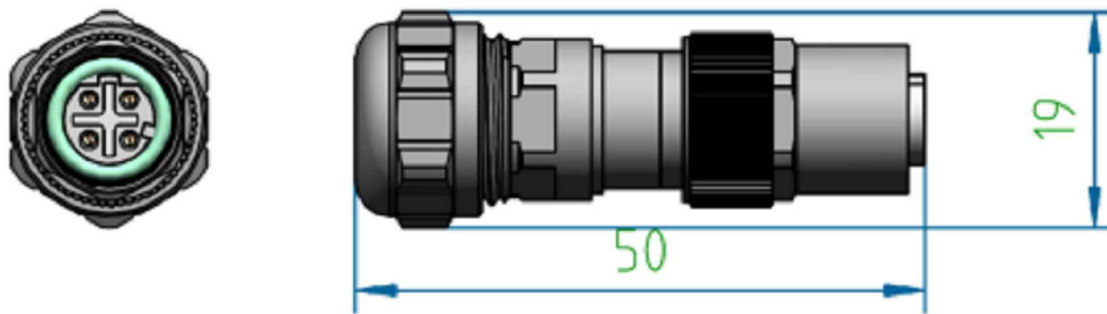
M12 D-4 FEMALE CABLE CLAMP RANGE FROM 5.5-9mm
