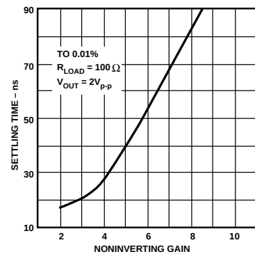
Figure 17. Settling Time vs. Noninverting Gain
