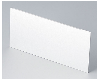
B6132111 Front panel Aluminum matt anodized 3.60"x1.71"x0.06"
