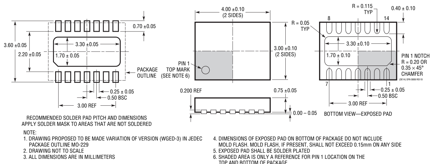
DE Package 14-Lead Plastic DFN (4mm × 3mm) (Reference LTC DWG # 05-08-1708 Rev B)
