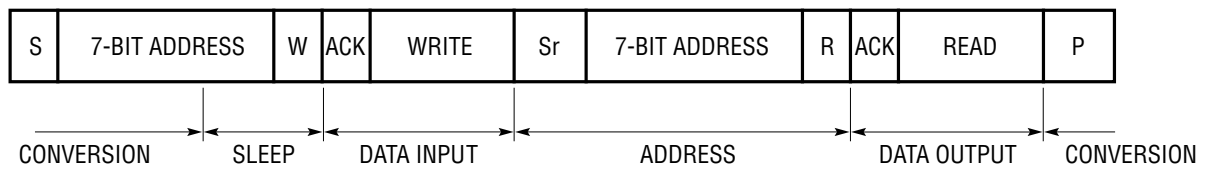
Figure 8. Write, Read, START Conversion
