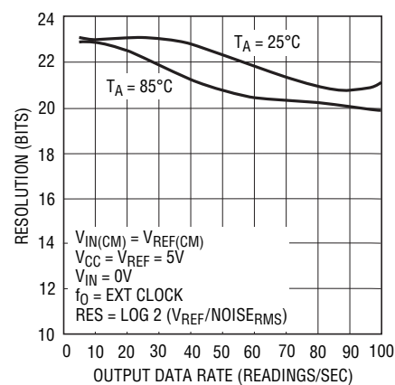
Figure 32. Resolution ( \text{Noise}_{\text{RMS}} \leq 1 \text{ LSB} ) vs Output Data Rate and Temperature
