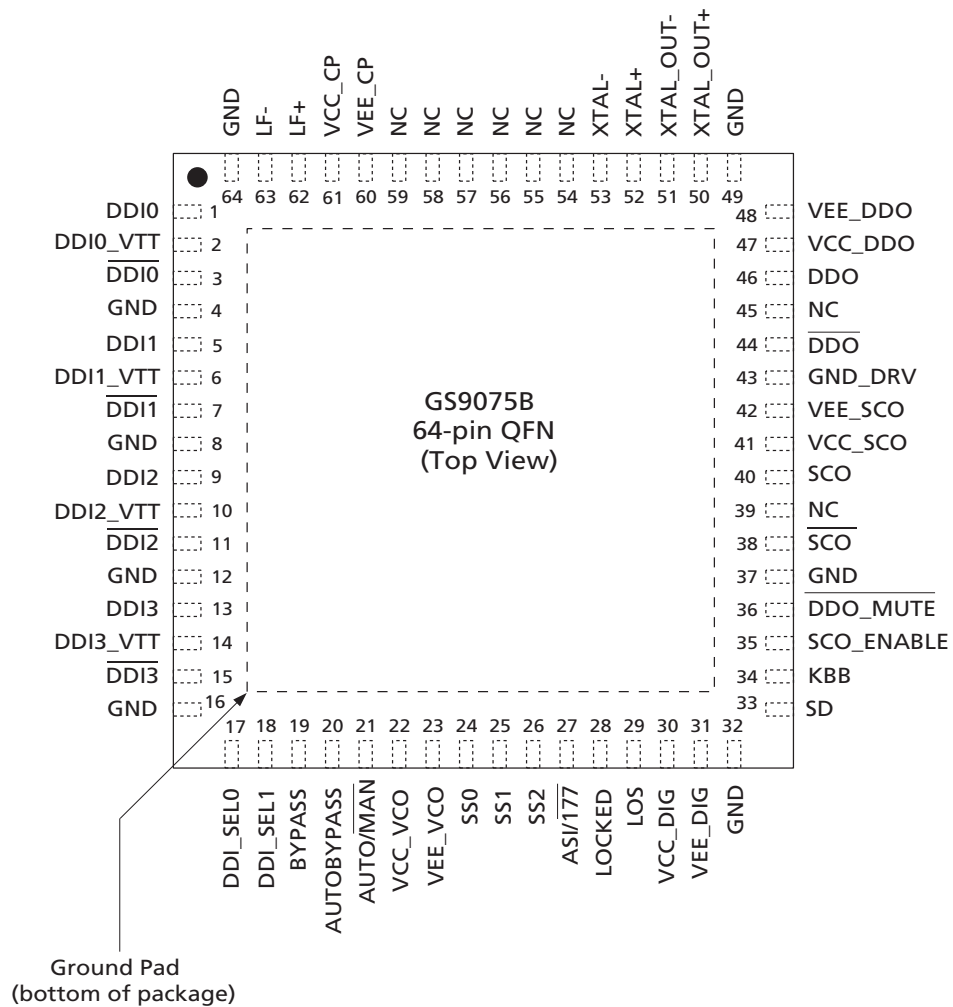
Figure 1-2: 64-Pin QFN
