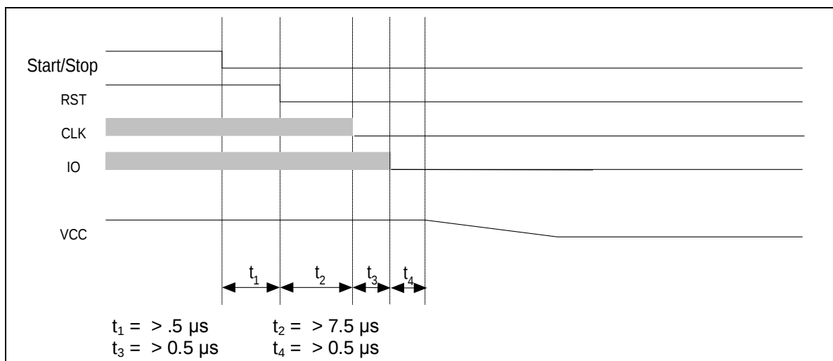
Figure 9: Deactivation Sequence
