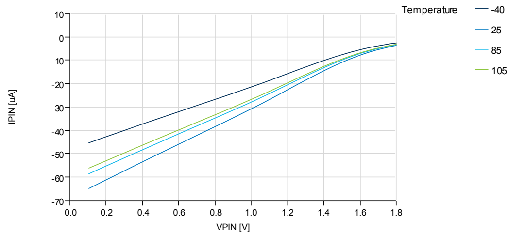
Figure 37-23.I/O pin pull-up resistor current vs. input voltage. V_{CC} = 1.8V .
