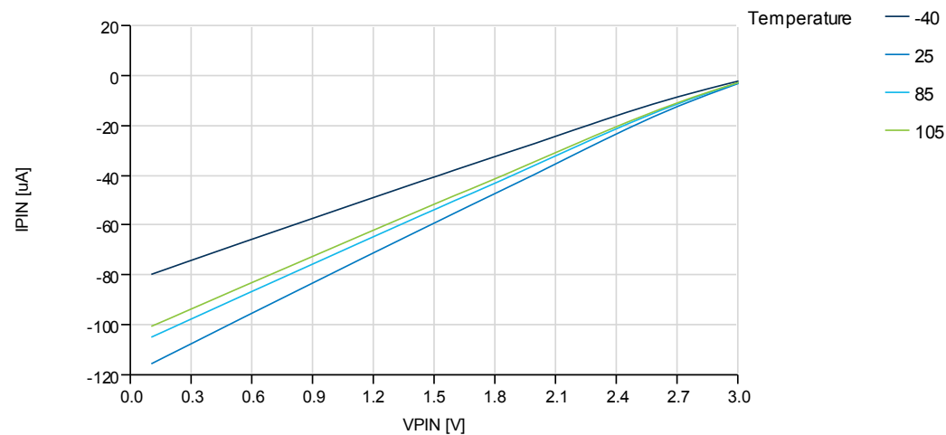
Figure 37-24.I/O pin pull-up resistor current vs. input voltage. V_{CC} = 3.0V .
