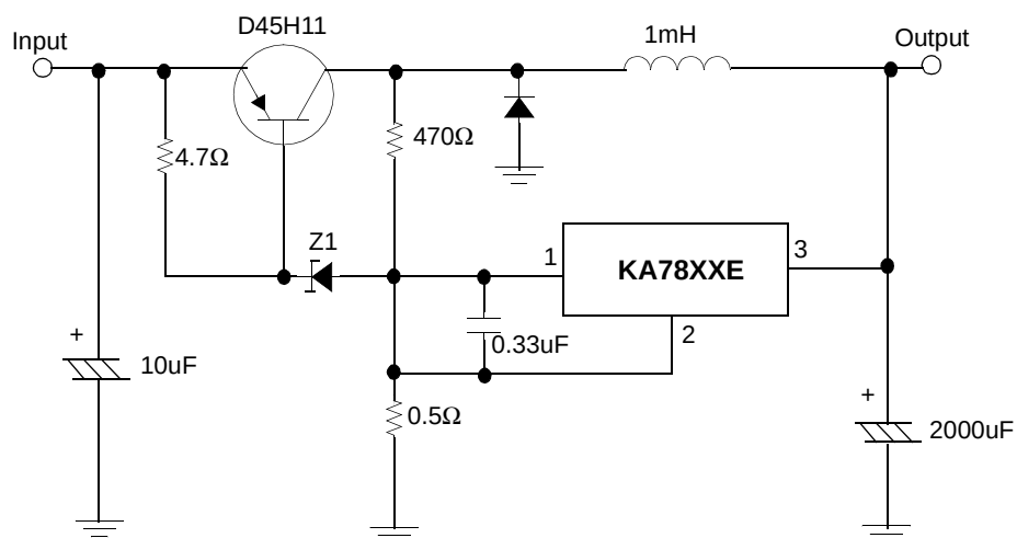
Figure 17. Switching Regulator
