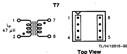
FIGURE 15. Coilcraft S6000-A
