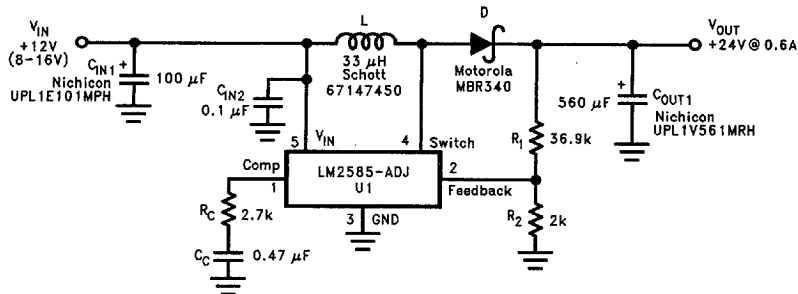
FIGURE 35. +12V to +24V Boost Regulator
