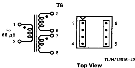
FIGURE 25. Renco RL-5533
