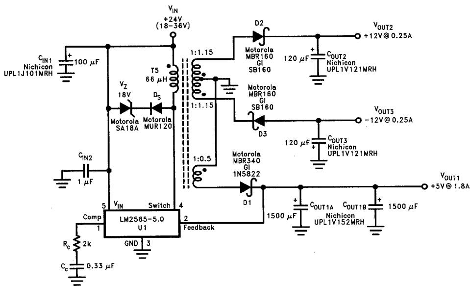
FIGURE 12. Triple-Output Flyback Regulator
