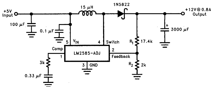
FIGURE 38. Boost Regulator
