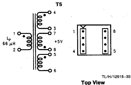
FIGURE 18. Coilcraft Q4338-B
