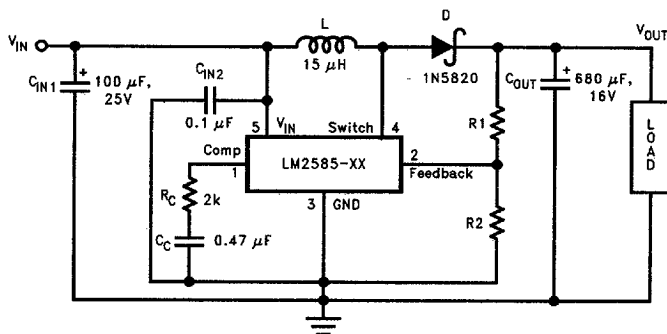
FIGURE 3. LM2585-12 and LM2585-ADJ
