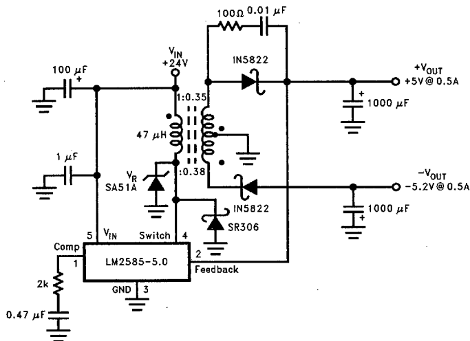
FIGURE 39. Flyback Regulator
