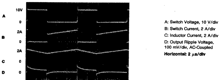
FIGURE 31. Switching Waveforms
