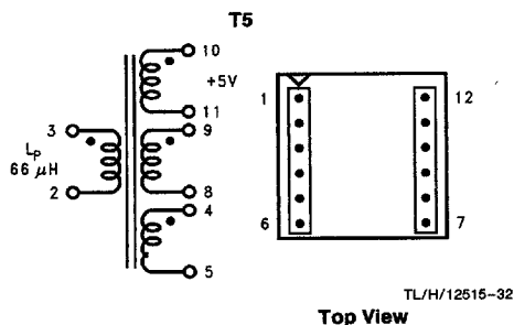
FIGURE 17. Coilcraft Q4437-B (Surface Mount)
