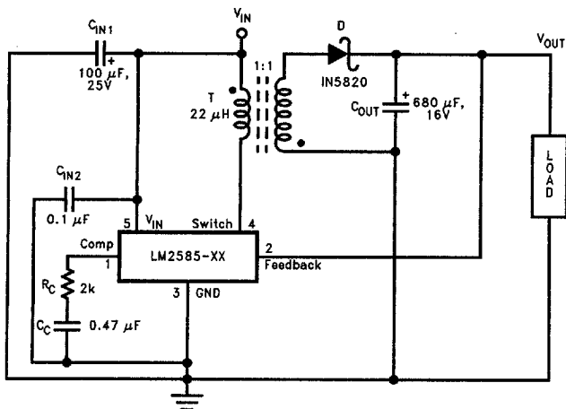
FIGURE 2. LM2585-3.3 and LM2585-5.0
