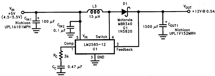
FIGURE 33. +5V to +12V Boost Regulator
