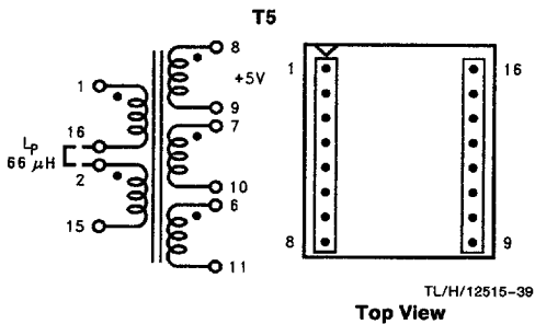
FIGURE 23. Pulse PE-68413 (Surface Mount)
