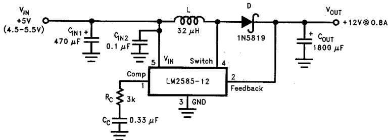
FIGURE 30. 12V Boost Regulator
