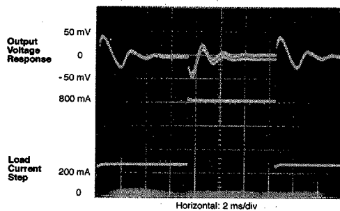
FIGURE 6. V_{OUT} Load Current Step Response
