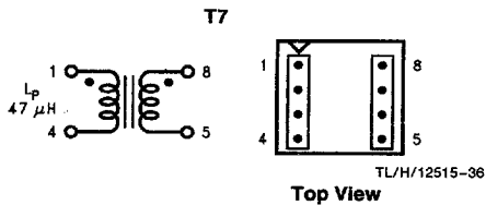
FIGURE 21. Pulse PE-68482
