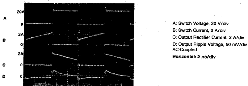
FIGURE 5. Switching Waveforms
