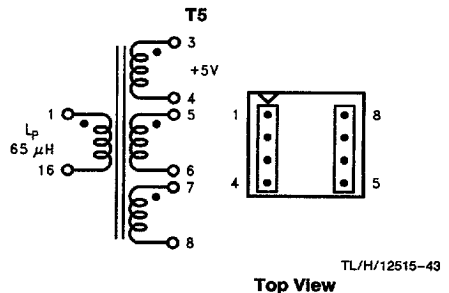
FIGURE 26. Renco RL-5532
