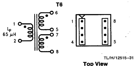
FIGURE 16. Coilcraft Q4339-B
