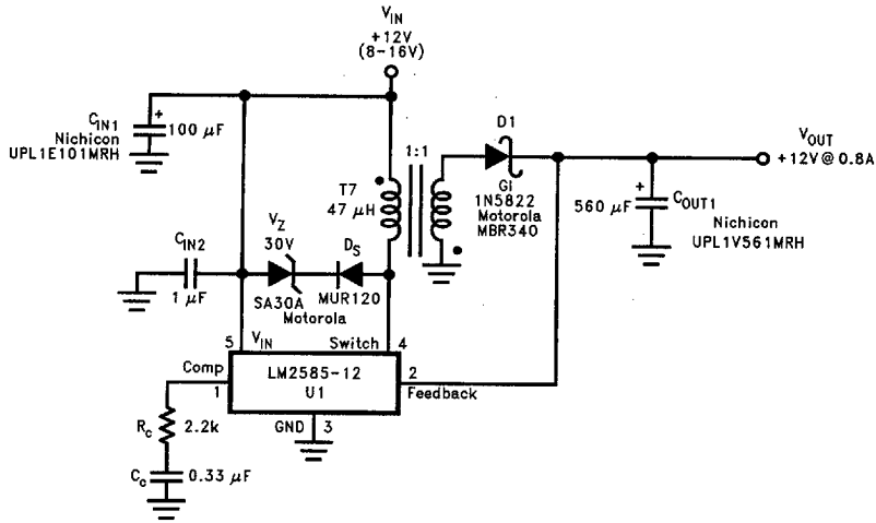
FIGURE 9. Single-Output Flyback Regulator
