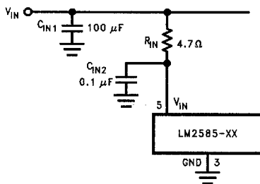
FIGURE 40. Input Line Filter
