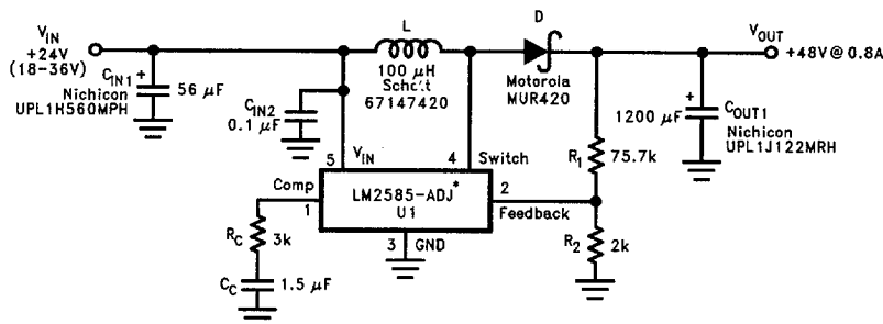
FIGURE 37. +24V to +48V Boost Regulator
