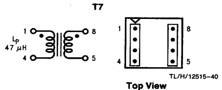
FIGURE 24. Renco RL-5751
