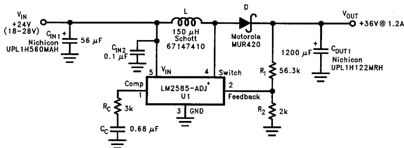
FIGURE 36. +24V to +36V Boost Regulator
