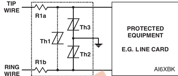
Figure 15. Protection Module
