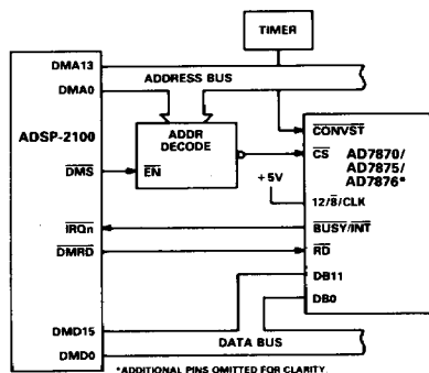
Figure 17. ADSP-2100 Parallel Interface
