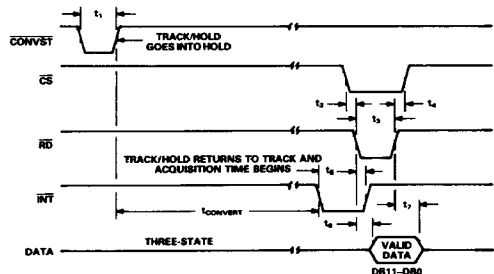
Figure 9. Mode 1 Timing Diagram, 12-Bit Parallel Read
