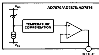
Figure 3. Reference Circuit
