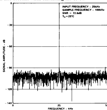
Figure 13. FFT Plot
