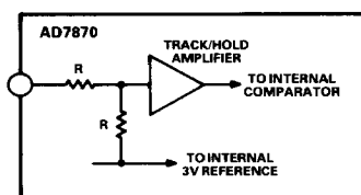
Figure 5a. AD7870 Analog Input
