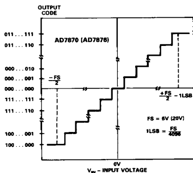
Figure 6. AD7870/AD7876 Transfer Function
