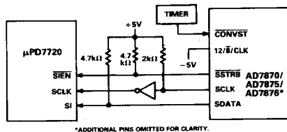
Figure 22. NEC7720 Serial Interface
