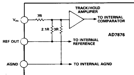
Figure 5b. AD7876 Analog Input
