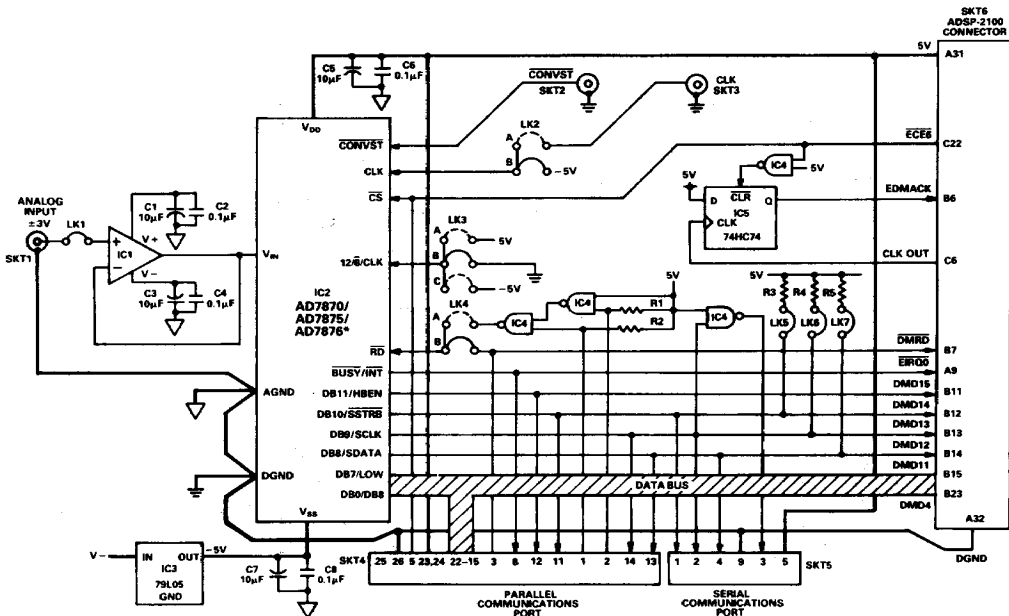
Figure 28. Data Acquisition Circuit Using the AD7870/AD7875/AD7876
