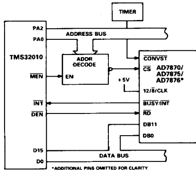
Figure 18. TMS32010 Parallel Interface
