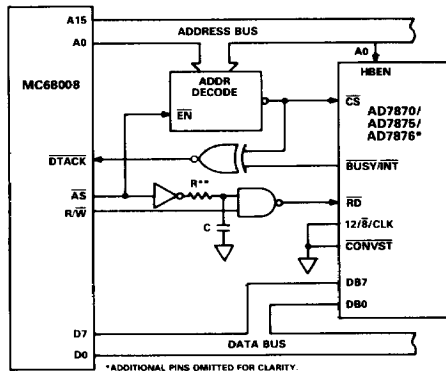
Figure 20. MC68008 Byte Interface
