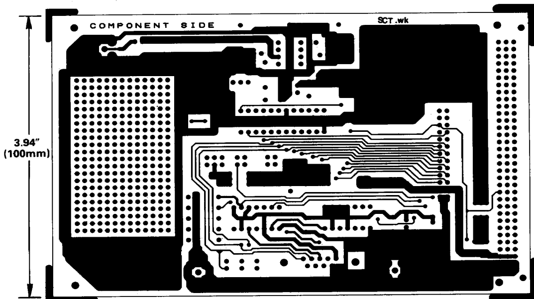
Figure 30. PCB Component Side Layout for Figure 28
