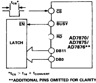
Figure 25. Stand-Alone Operation
