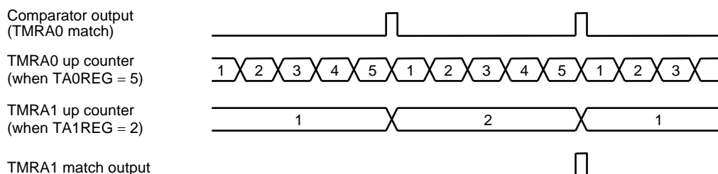
Figure 3.12.17 TMRA1 Count Up on Signal from TMRA0
