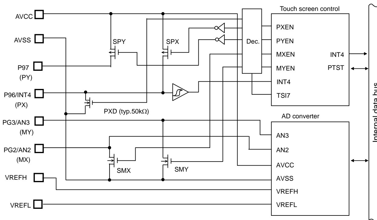
Figure 3.19.2 Internal block diagram of TSI
