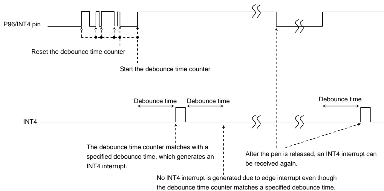
Figure 3.19.4 Timing diagram of debounce circuit
