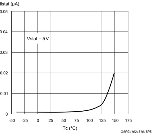
Figure 19. Status leakage current
