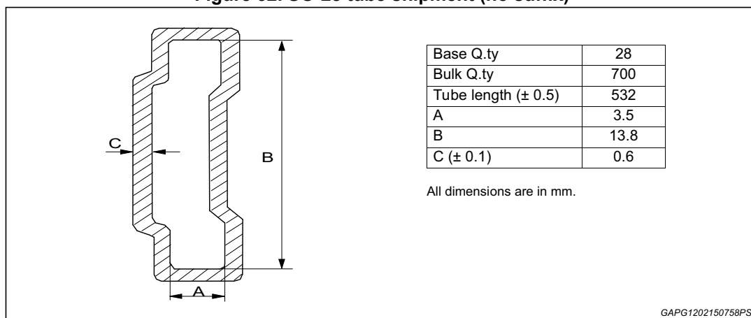
Figure 32. SO-28 tube shipment (no suffix)
