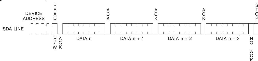
Figure 7-3. Sequential Read
