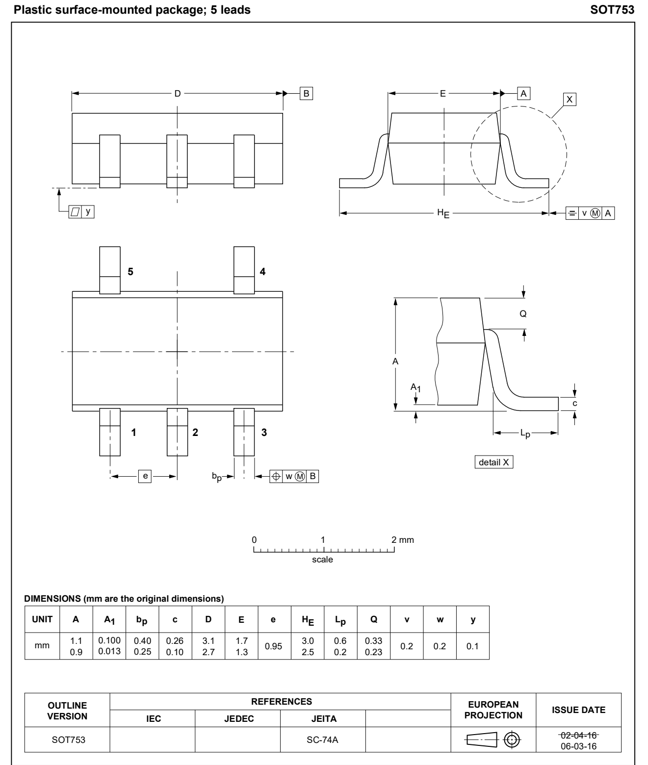
Fig. 9. Package outline SOT753 (SC-74A)
