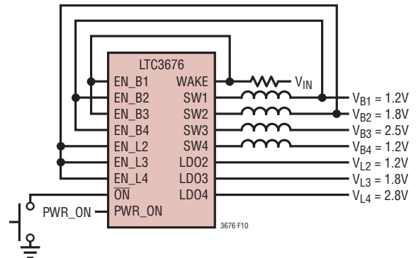
Figure 10. Pin-Strapped Power-On Sequence Application
