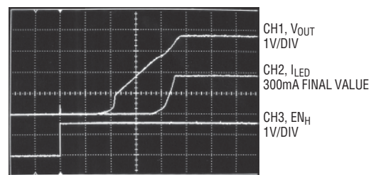
Start-Up Transient
