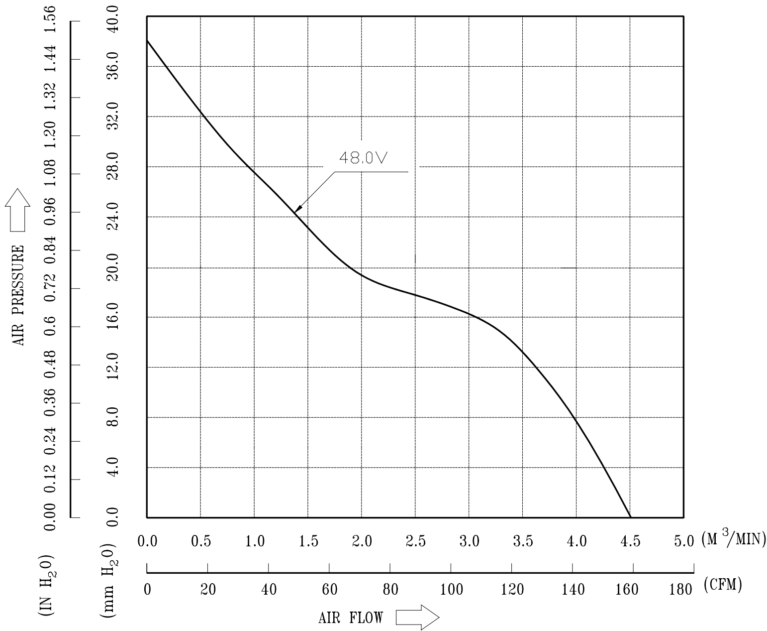
8. P & Q CURVE:
