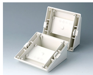
B4042847 Base S - desk-top/wall - ABS (UL 94 HB) off-white RAL 9002 4.84"x4.84"x2.09"
