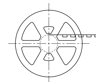
PLASTIC REEL
