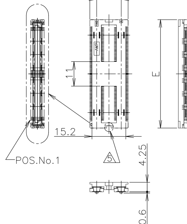
CONNECTOR DETAIL
