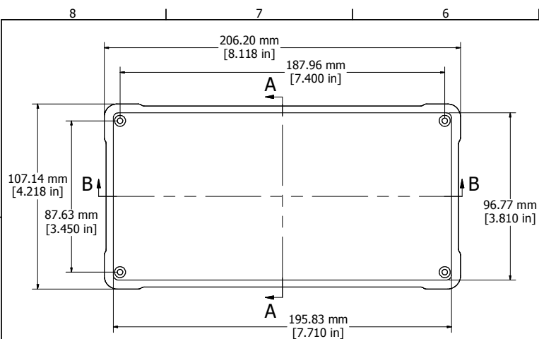
ASSEMBLY - TOP VIEW
