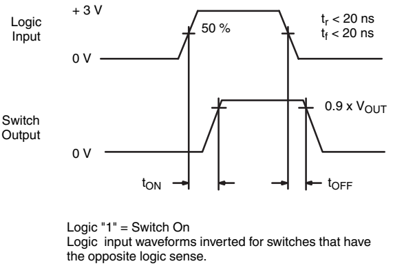
Figure 1. Switching Time
