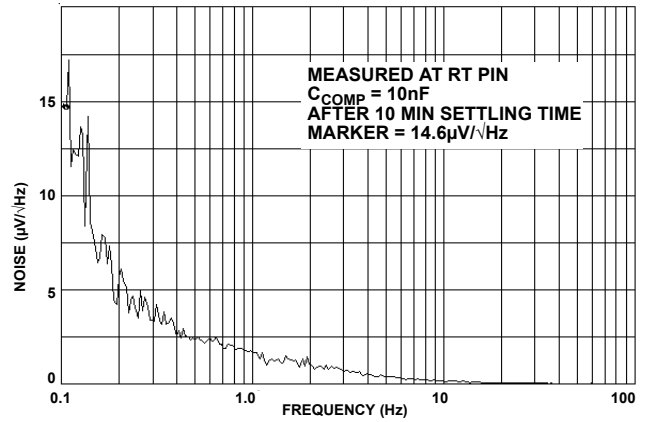
FIGURE 3. NOISE LEVEL AT R_{TH} INPUT IN CLOSE LOOP APPLICATION 2 \mu V/\sqrt{Hz} @ 1Hz
