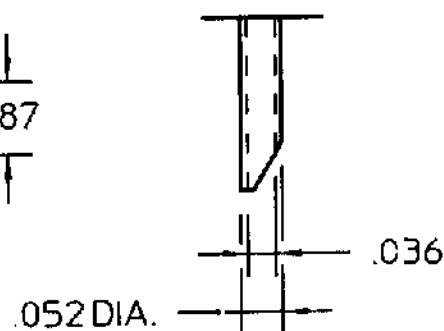
SOLDER CUP TERMINAL
