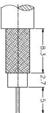
RECOMMENDED CABLE STRIPPING DIM'S
