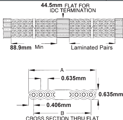
Typical 125-3001 Laminated Pair Solid Core Planar Cable (figure shown above) Type 125-3007, same as 125-3001 shown above except with stranded cores (7/38AWG)
