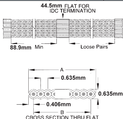
Typical 425-3006 Loose Pair Stranded Core TnF Planar Cable
