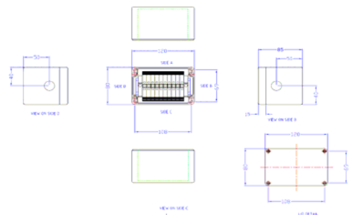
JB-FT10 Drawing
