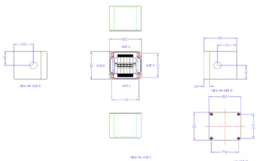
JB-FT5 Drawing
