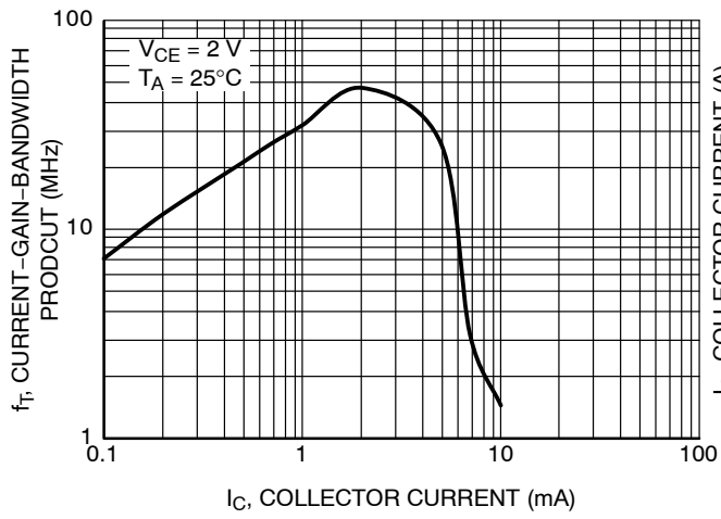
Figure 4. Current-Gain-Bandwidth Product
