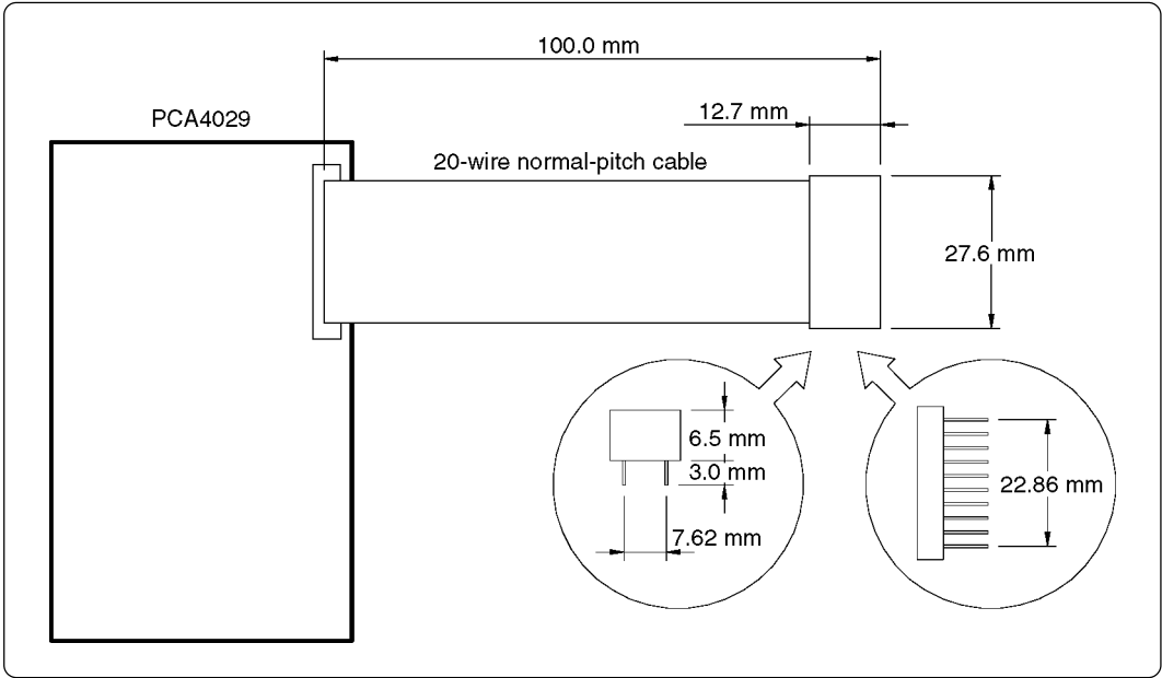
Figure 8.1 External dimensions of 20-pin pin header
