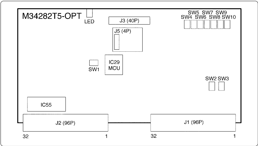
Figure 4.2 Switch locations
